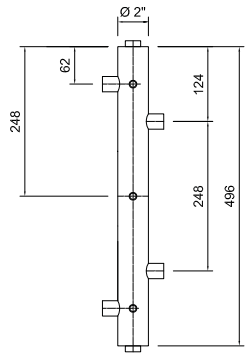
COD. ACC7400170 Separador Hidráulico 2", 2VX1" + 2VX1" + 5VX1/2"
